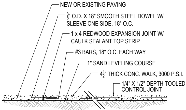
SECTION A ELEVATION - NTS
